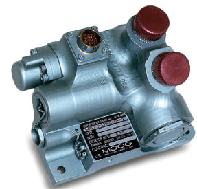
Thermal Bypass Valve
